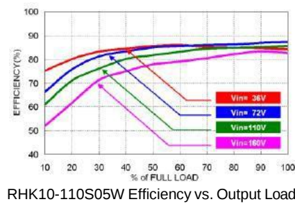
RHK10-110S05W Efficiency vs. Output Load
