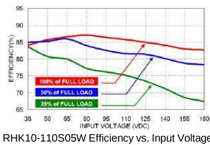
RHK10-110S05W Efficiency vs. Input Voltage
