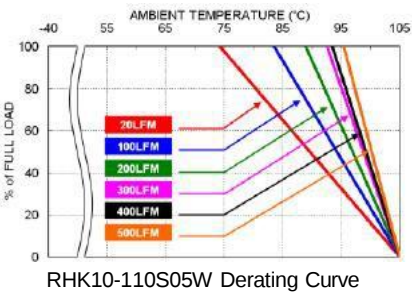
RHK10-110S05W Derating Curve
