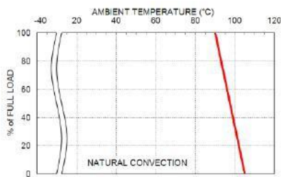
SDS(H)01-48S05 Derating Curve
