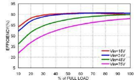
SDS(H)02-48S05W Efficiency vs. Output Current
