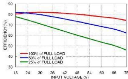
SDS(H)02-48S05W Efficiency vs. Input Voltage
