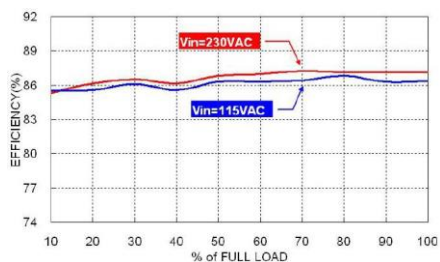
TAC15US12B Efficiency vs. Output Load
