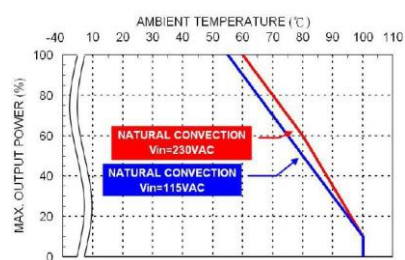
Derating Curve vs. Ambient Temperature TAC15USxxB xx=3P3/05/7P5/09/12/15/18 Connector Option : ( -M / -T / -D )
