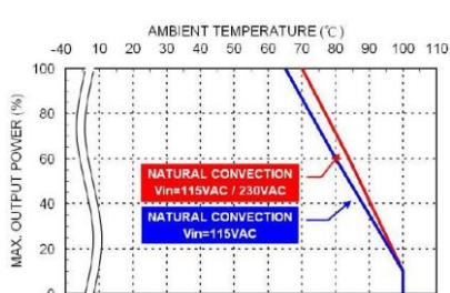
Derating Curve vs. Ambient Temperature TAC15USxxB xx=24/28/36/48/53 Connector Option : ( -M / -T / -D )
