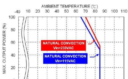
Derating Curve vs. Ambient Temperature TAC15USxxB xx=24/28/36/48/53 Connector Option : (□: JST)
