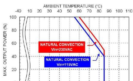
Derating Curve vs. Ambient Temperature TAC15USxxB xx=3P3/05/7P5/09/12/15/18 Connector Option : (□: JST)
