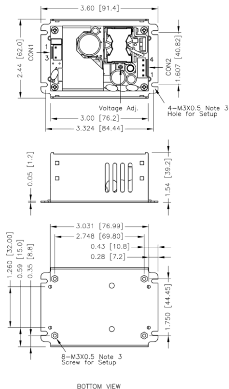
BOTTOM VIEW
