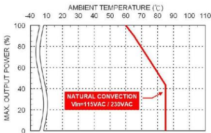
TAD30US24B-P Derating Curve vs. Ambient Temperature
