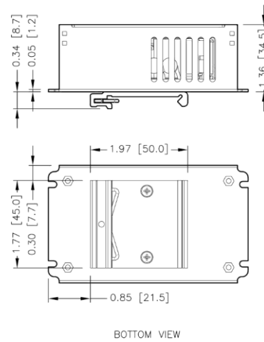
BOTTOM VIEW
