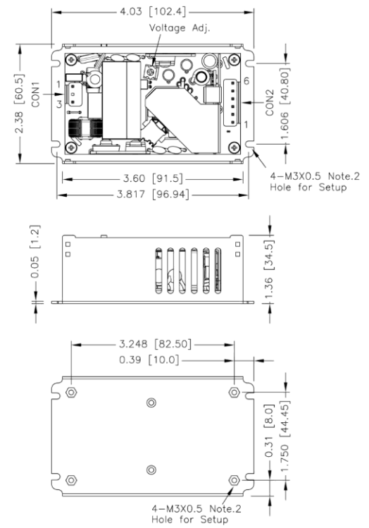
BOTTOM VIEW
