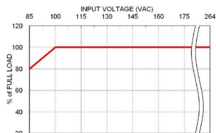
T1: F150 Derating Curve vs. Input Voltage
