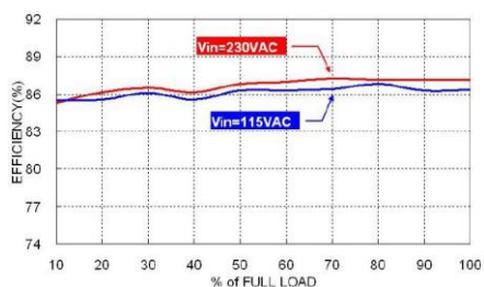
TSC15US12B Efficiency vs. Output Load
