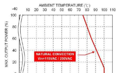
Derating Curve vs. Ambient Temperature TSC15USxxB xx=24/28/36/48/53 Connector Option : ( -M / -T / -D )
