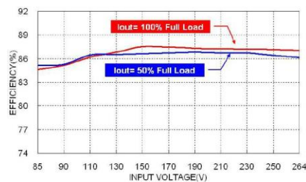
TSC15US12B Efficiency vs. Input Voltage
