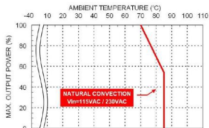
Derating Curve vs. Ambient Temperature TSC15USxxB xx=3P3/05/7P5/09/12/15/18 Connector Option : (□: JST)
