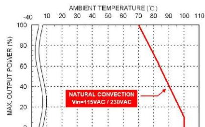
Derating Curve vs. Ambient Temperature TSC15USxxB xx=3P3/05/7P5/09/12/15/18 Connector Option : ( -M / -T / -D )
