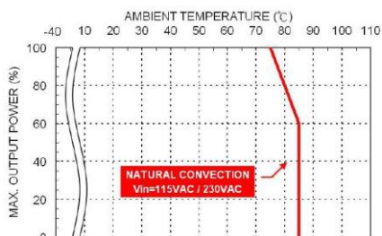
Derating Curve vs. Ambient Temperature TSC15USxxB xx=24/28/36/48/53 Connector Option : (□: JST)
