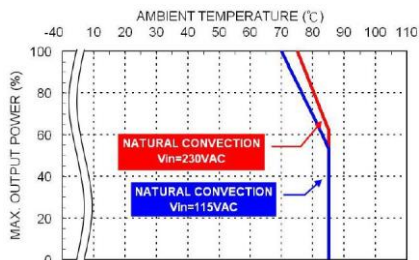
Derating Curve vs. Ambient Temperature TSD30USxxB xx=12/15/24/28/36/48/53 Connector Option : ( □ : JST )
