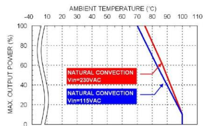
Derating Curve vs. Ambient Temperature TSD30USxxB xx=12/15/24/28/36/48/53 Connector Option : ( -M / -T / -D )
