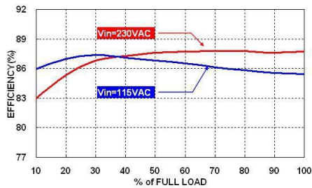
TSD30US24B Efficiency vs. Output Load
