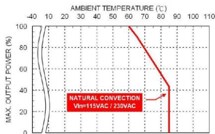
Derating Curve vs. Ambient Temperature TSD30USxxB xx=3P3/05/7P5/09/121/151/18 Connector Option : ( □ : JST )
