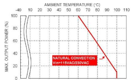
Derating Curve vs. Ambient Temperature TSD30USxxB xx=3P3/05/7P5/09/121/151/18 Connector Option : ( -M / -T / -D )
