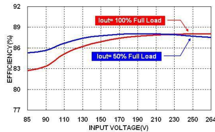
TSD30US24B Efficiency vs. Input Voltage
