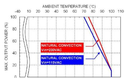
Derating Curve vs. Ambient Temperature TSD30USxxB xx=12/15/24/28/36/48/53 Connector Option : ( -M / -T / -D )
