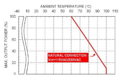
Derating Curve vs. Ambient Temperature TSD30USxxB xx=3P3/05/7P5/09/121/151/18 Connector Option : ( -M / -T / -D )
