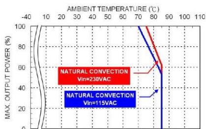
Derating Curve vs. Ambient Temperature TSD30USxxB xx=12/15/24/28/36/48/53 Connector Option : (□: JST)
