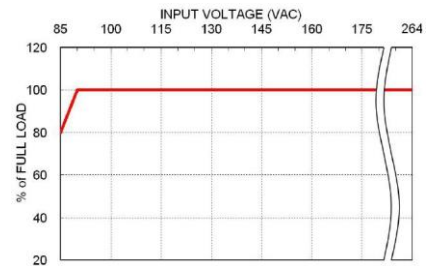
TSD65 Derating Curve vs. Input Voltage
