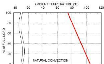
UDS(H)02-24S05 Derating Curve
