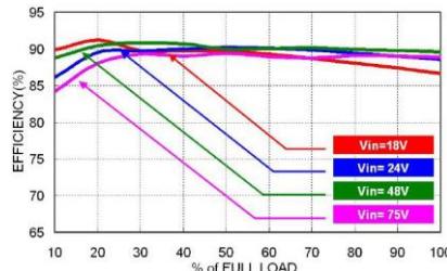
WAF300-48S12W Efficiency vs. Output Load
