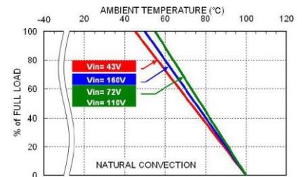
WAF300-110S □□ W Derating Curve
