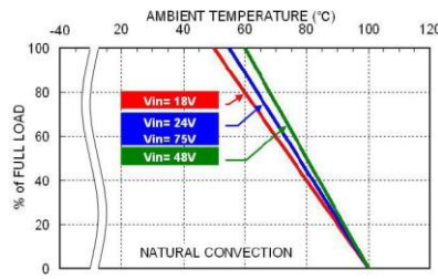
WAF300-48S □□ W Derating Curve With 3U Iron Base-Plate
