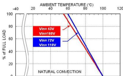
WAF300-110S □□ W Derating Curve With 3U Iron Base-Plate
