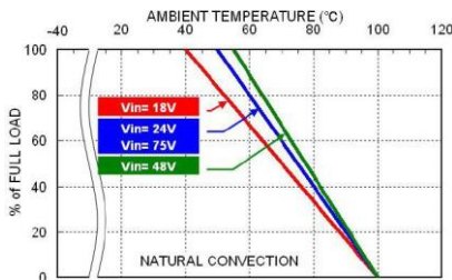
WAF300-48S □□ W Derating Curve
